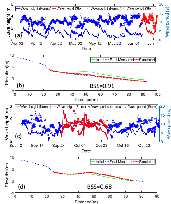
Figure 1 - (a) and (c): Wave conditions during the simulation periods. (b) and (d): Comparison between simulated and measured cross-shore beach profiles.
